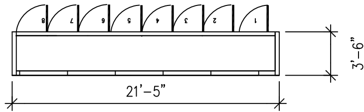
FLOOR PLAN
